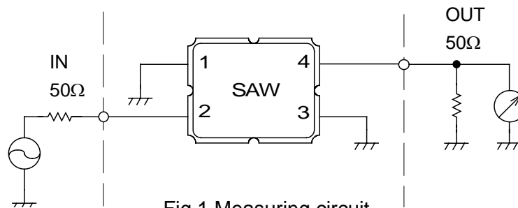
Fig.1 Measuring circuit
